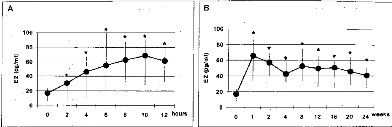
FIG. 1. Mean estradiol ( E_2 ) serum levels after insertion of one 25-mg E_2 implant (Rischle) in postmenopausal women ( n = 15 ) at regular intervals on the day of insertion (A) and at follow-up visits during a period of 24 weeks (B). Vertical lines represent the 25 and 75 percentiles. *, statistically significant change compared with baseline ( p < 0.05 ).
